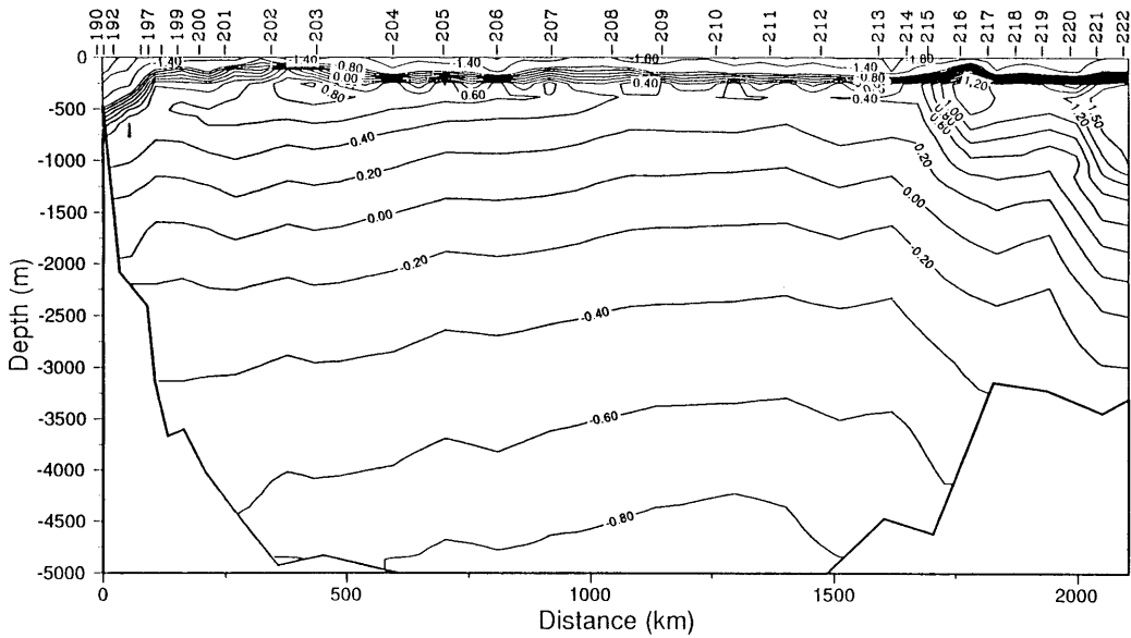
Figure 5: Potential temperature distribution on the meridional section of "Polarstern". Numbers on the top line indicate hydrographic stations
